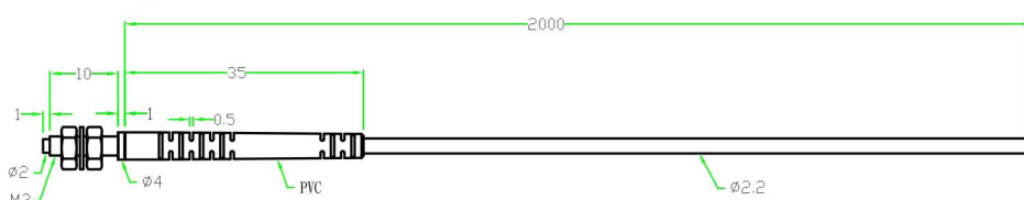
Fiber Optic Cable Through Beam Model : FOS300T, Sn : 300mm
